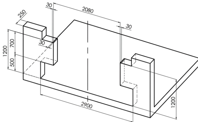
PIT DIMENSIONS FORMWORK BOX
